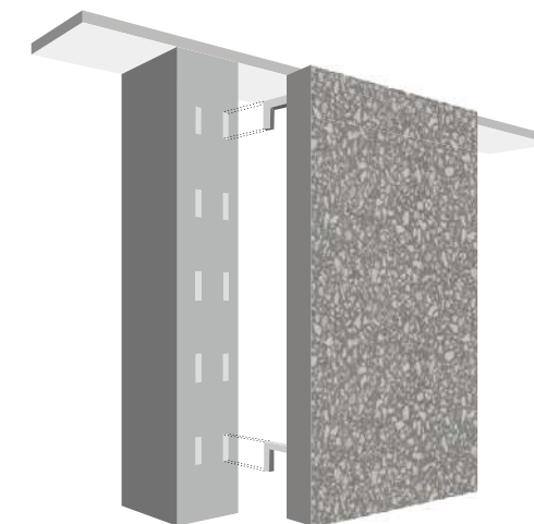
Hook Type
